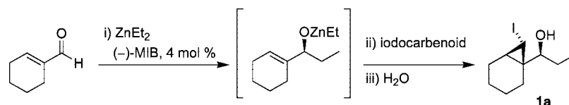
Scheme 4. Asymmetric Addition/Diastereoselective Iodocyclopropanation Optimization (see Table 1)
