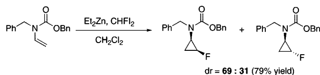
Scheme 2. Diastereoselective Fluorocyclopropanation
